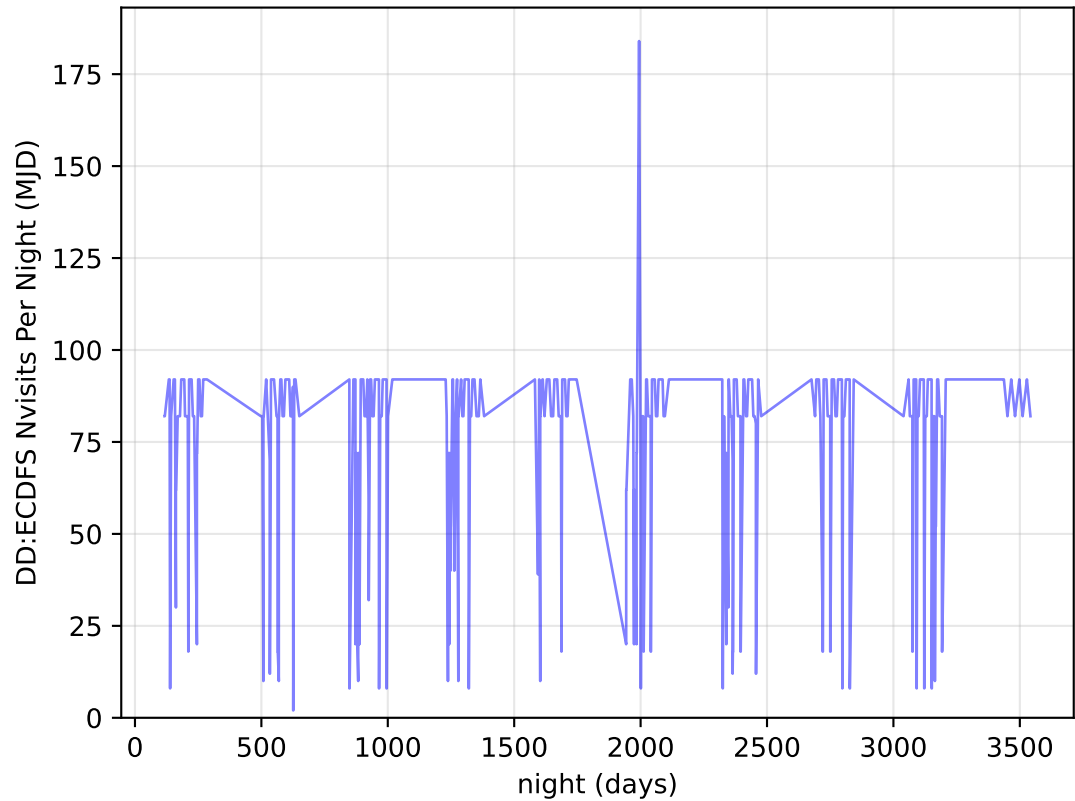
ddf_acor_sf20_lsf30_lsr10_v3.4_10yrs all bands: DD:ECDFS Nvisits Per Night
