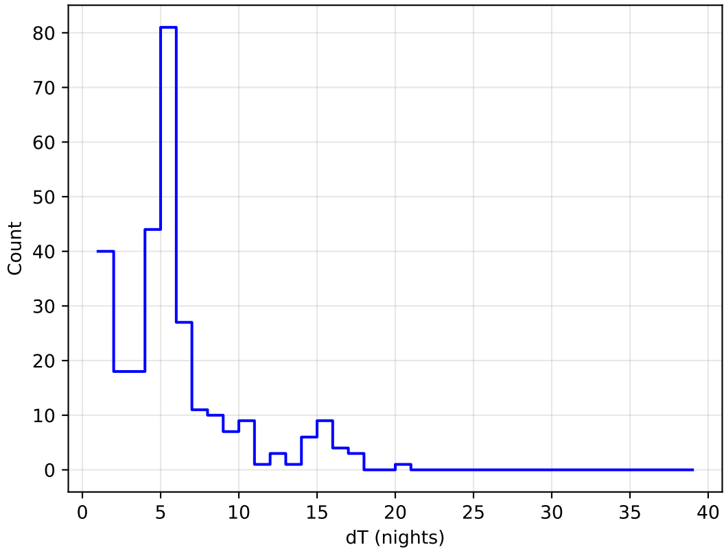
ddf_acor_sf20_lsf30_lsr10_v3.4_10yrs all bands: DD:ECDFS Delta Nights Histogram
