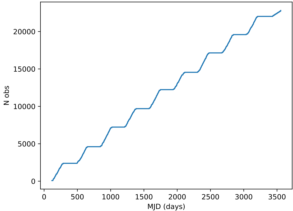
ddf_acor_sf20_lsf30_lsr10_v3.4_10yrs all bands: DD:ECDFS Cumulative NVisits
