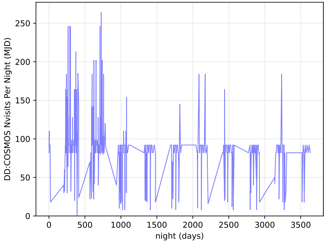
ddf_acor_sf20_lsf30_lsr10_v3.4_10yrs all bands: DD: COSMOS Nvisits Per Night
