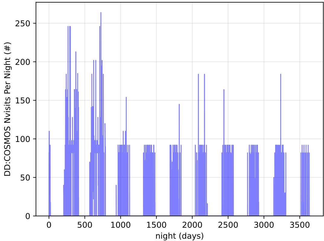
ddf_acor_sf20_lsf30_lsr10_v3.4_10yrs all bands: DD:COSMOS Nvisits Per Night
