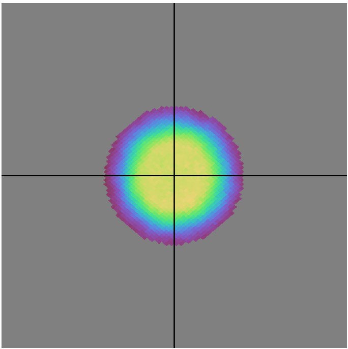
ddf_acor_sf20_lsf30_lsr10_v3.4_10yrs all bands: DD:COSMOS N Unique Nights
