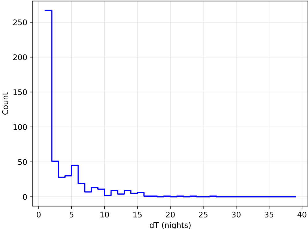
ddf_acor_sf20_Isf30_Isr10_v3.4_10yrs all bands: DD: COSMOS Delta Nights Histogram
