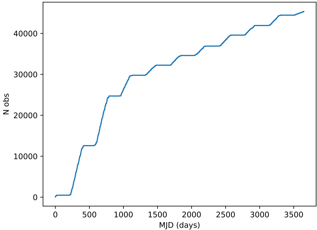
ddf_acor_sf20_lsf30_lsr10_v3.4_10yrs all bands: DD: COSMOS Cumulative NVisits
