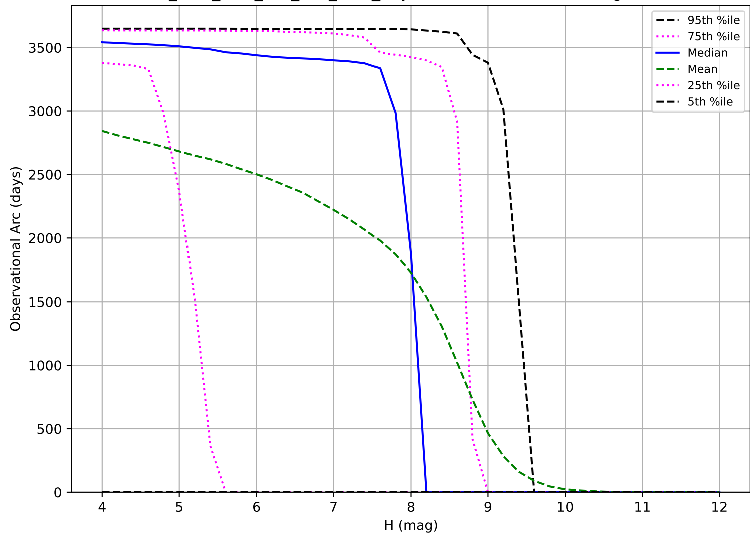
ddf_acor_sf20_lsf0_lsr0_v3.4_10yrs: Observational Arc Length TNO
