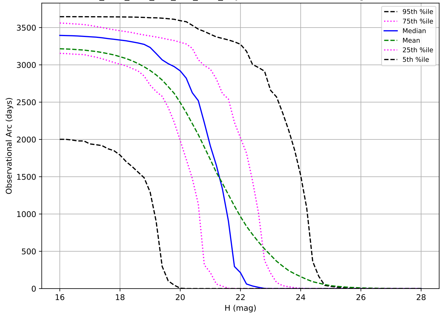
ddf_acor_sf20_lsf0_lsr0_v3.4_10yrs: Observational Arc Length PHA
