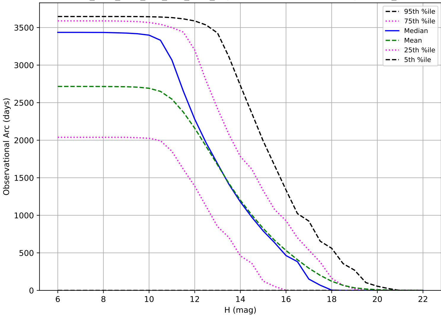
ddf_acor_sf20_lsf0_lsr0_v3.4_10yrs: Observational Arc Length OCC_r5
