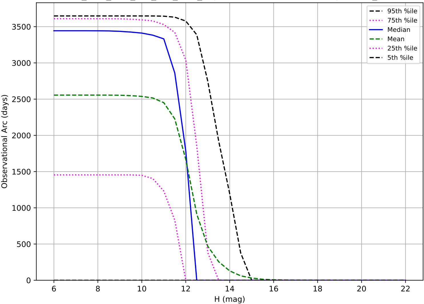
ddf_acor_sf20_lsf0_lsr0_v3.4_10yrs: Observational Arc Length OCC_r20
