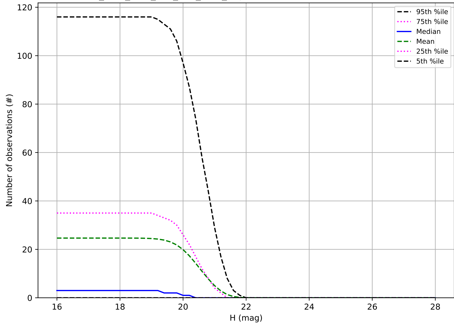
ddf_acor_sf20_lsf0_lsr0_v3.4_10yrs: Number of observations Vatira
