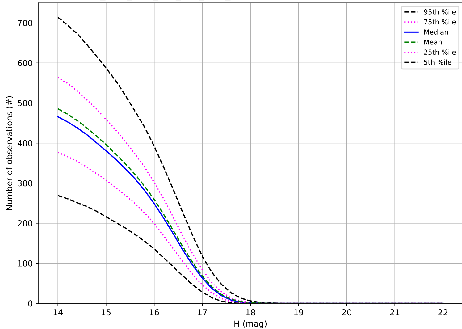
ddf_acor_sf20_lsf0_lsr0_v3.4_10yrs: Number of observations Trojan
