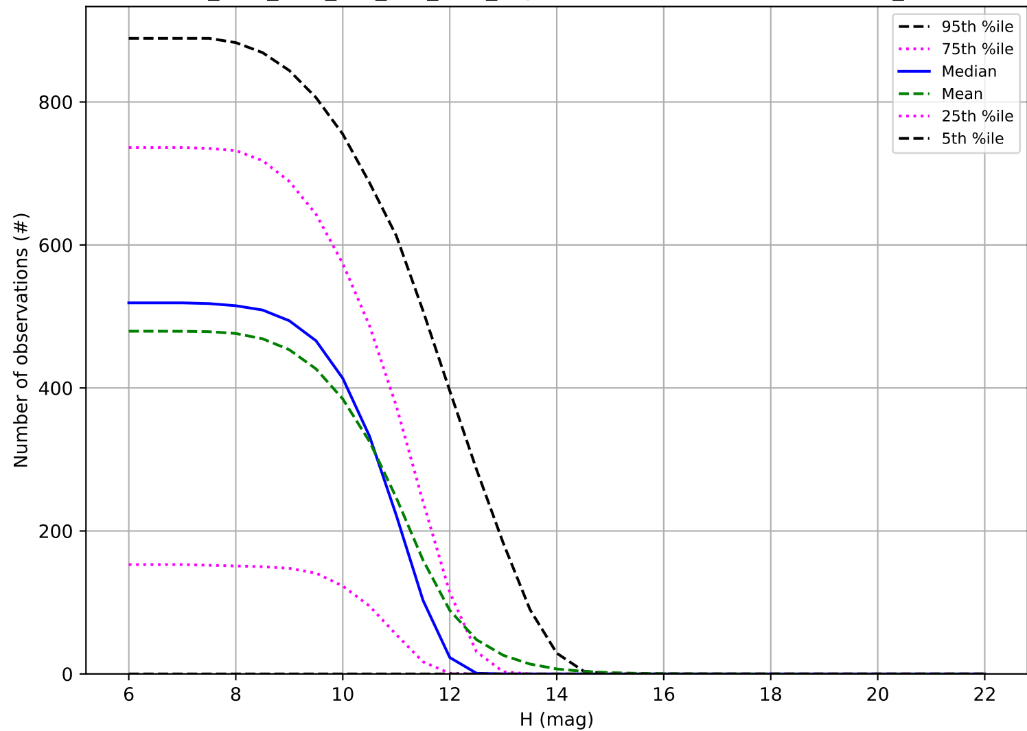
ddf_acor_sf20_lsf0_lsr0_v3.4_10yrs: Number of observations OCC_r20
