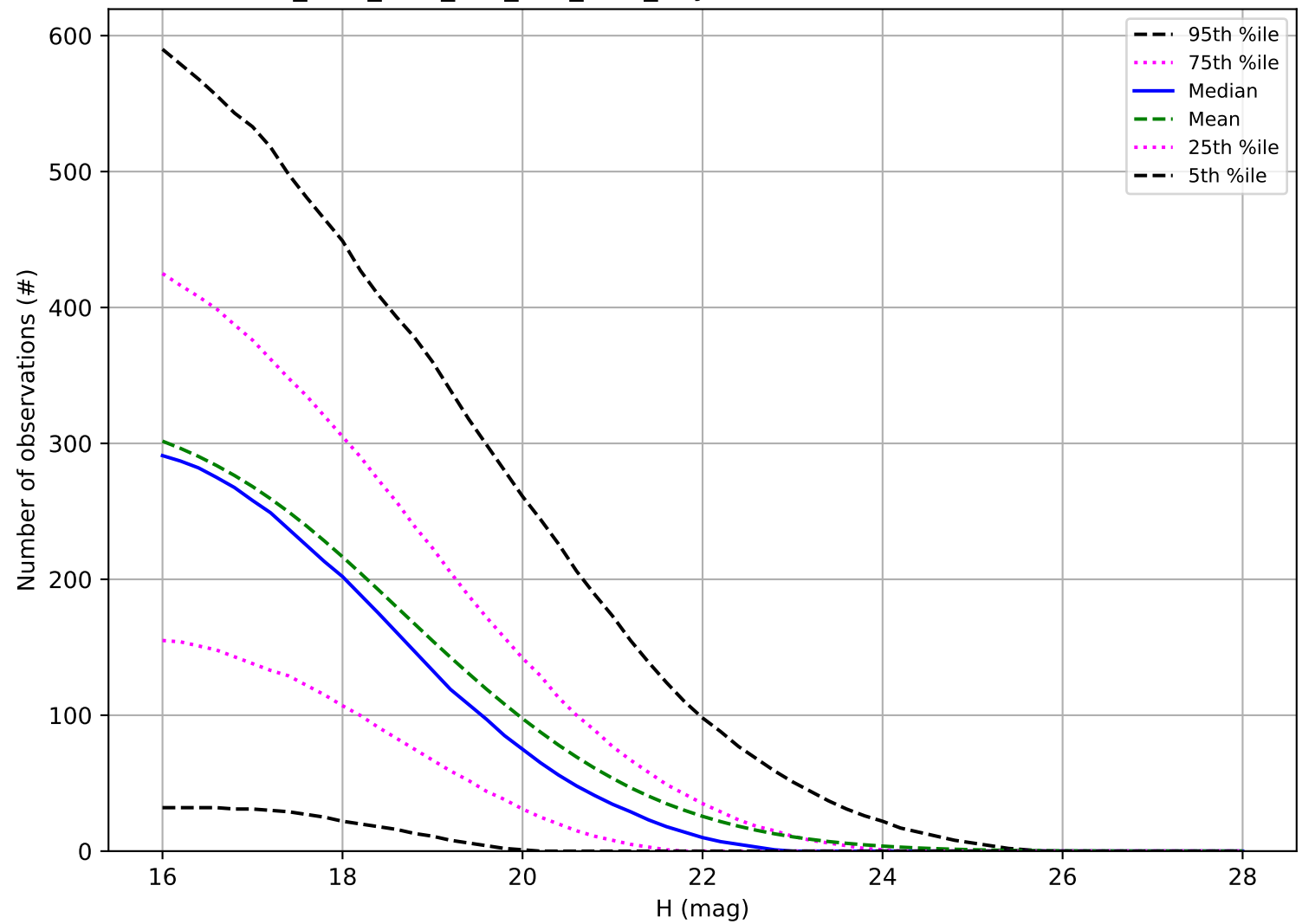
ddf_acor_sf20_lsf0_lsr0_v3.4_10yrs: Number of observations NEO
