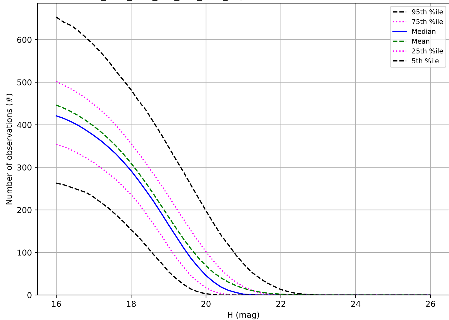
ddf_acor_sf20_lsf0_lsr0_v3.4_10yrs: Number of observations MBA
