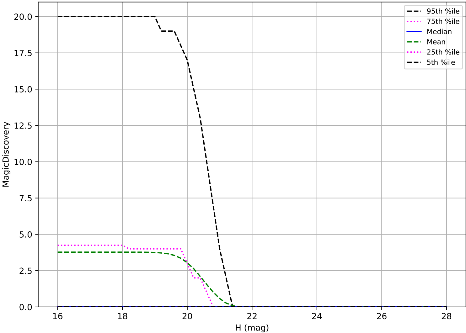
ddf_acor_sf20_lsf0_lsr0_v3.4_10yrs: Vatira 6 detections in 60 nights detection loss
