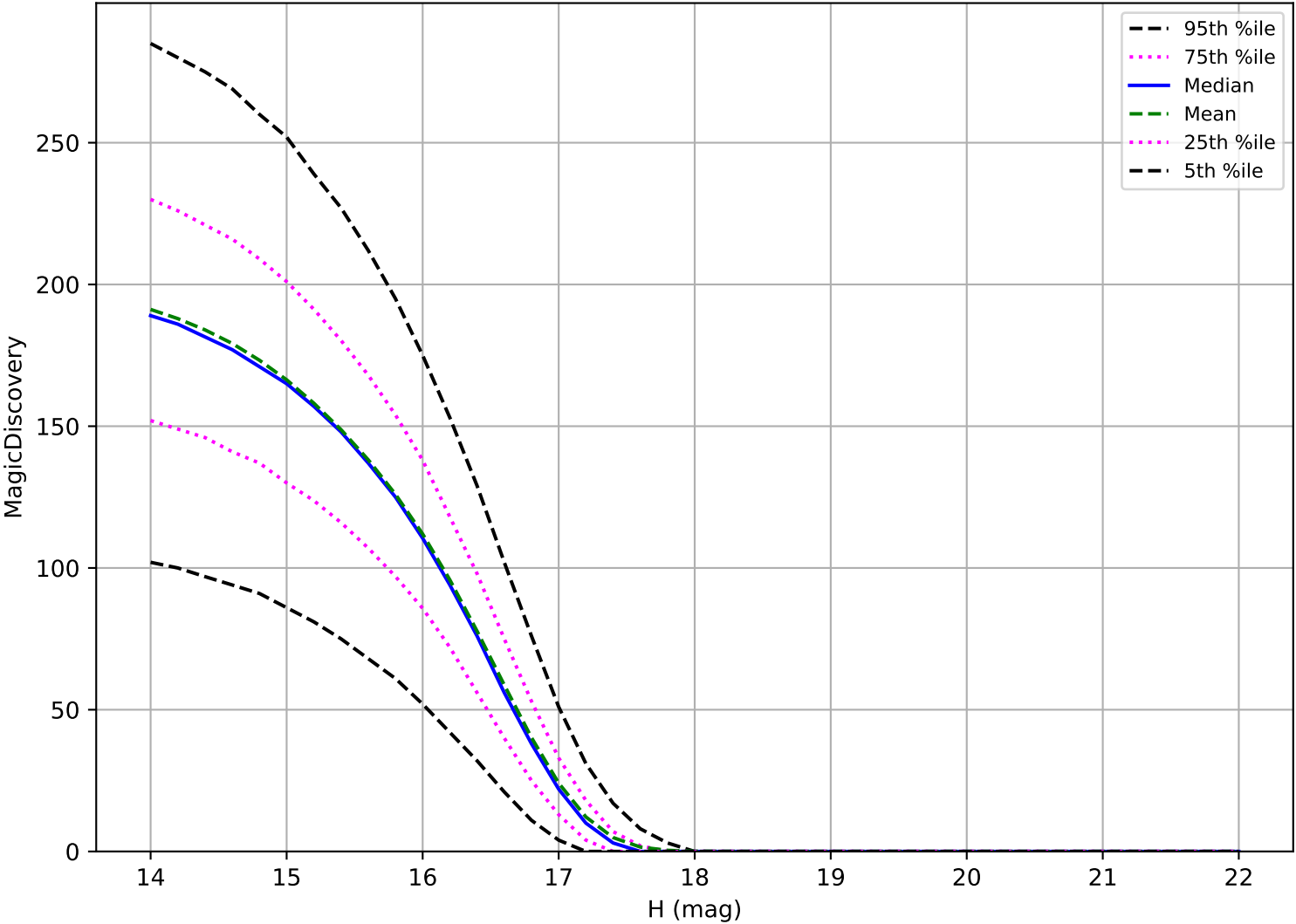
ddf_acor_sf20_lsf0_lsr0_v3.4_10yrs: Trojan 6 detections in 60 nights detection loss
