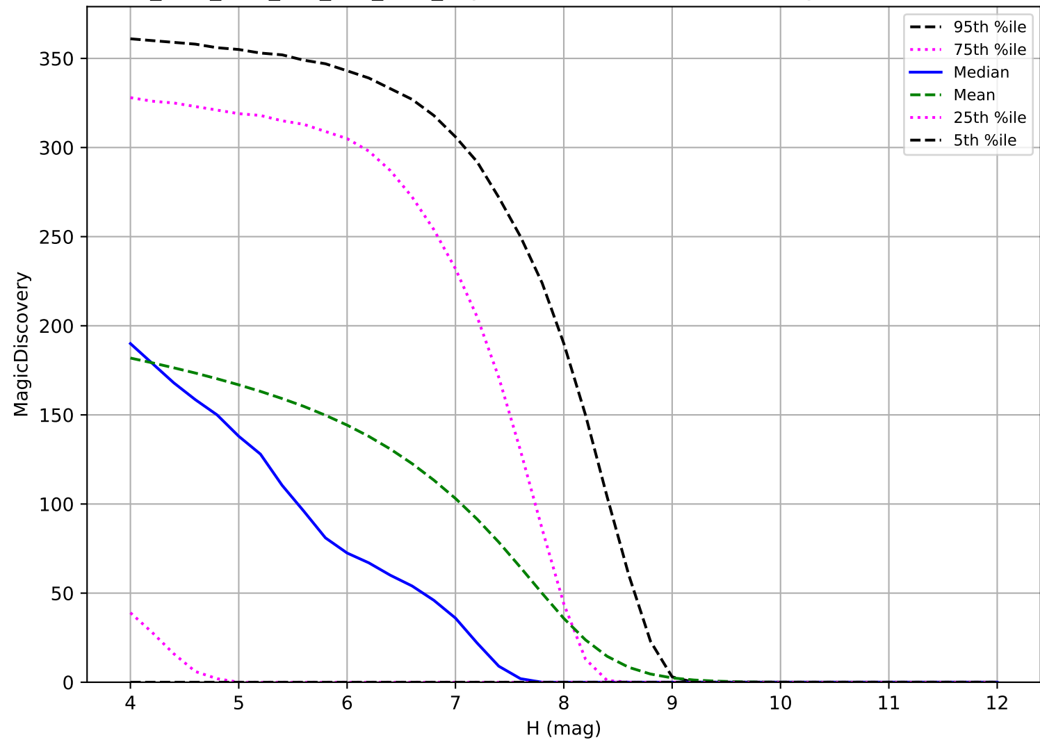
ddf_acor_sf20_lsf0_lsr0_v3.4_10yrs: TNO 6 detections in 60 nights detection loss
