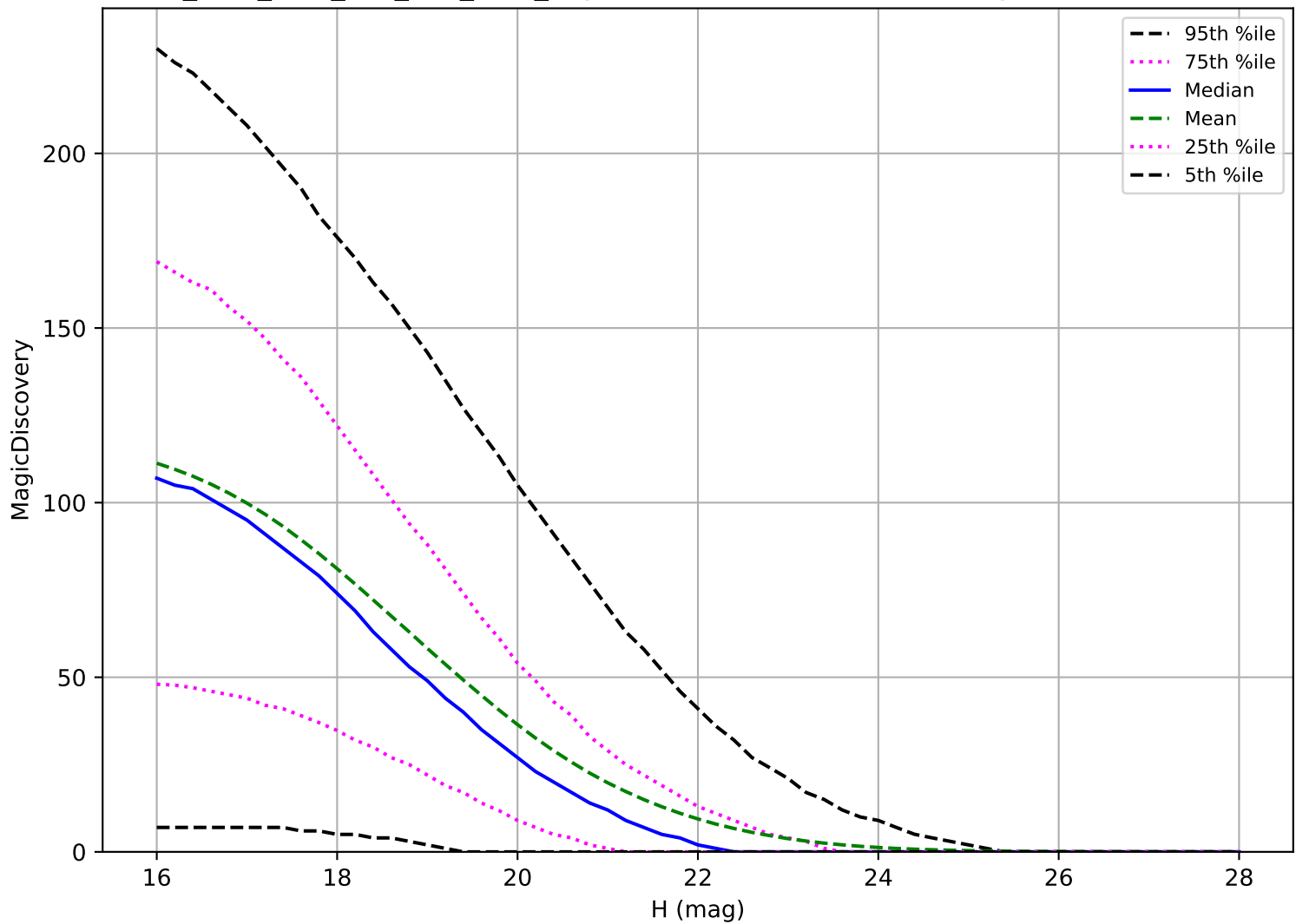
ddf_acor_sf20_lsf0_lsr0_v3.4_10yrs: PHA 6 detections in 60 nights detection loss
