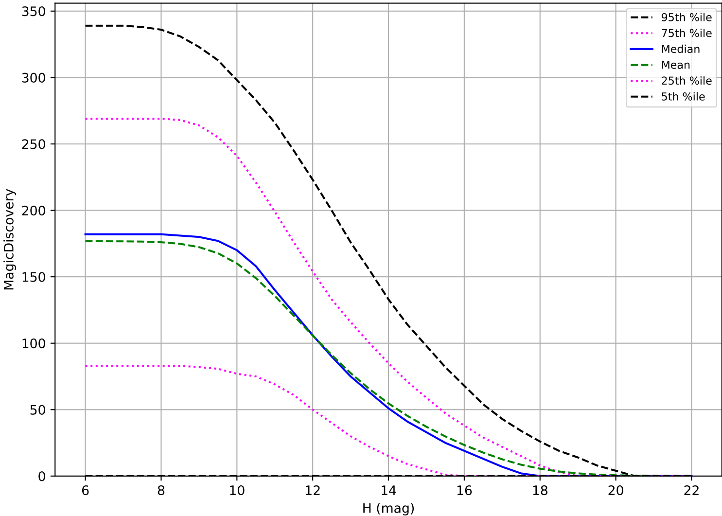
ddf_acor_sf20_lsf0_lsr0_v3.4_10yrs: OCC_r5 6 detections in 60 nights detection loss
