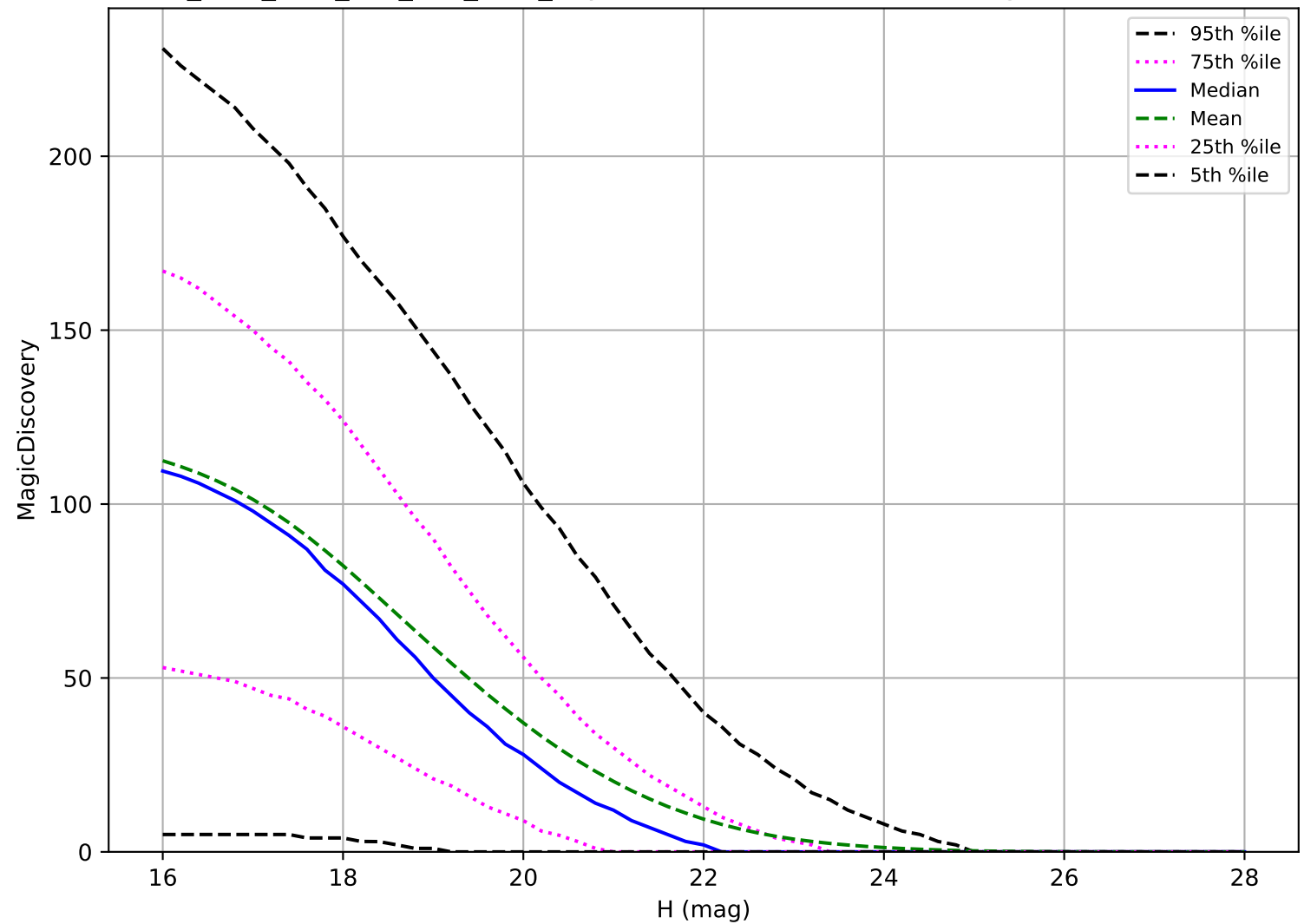
ddf_acor_sf20_lsf0_lsr0_v3.4_10yrs: NEO 6 detections in 60 nights detection loss
