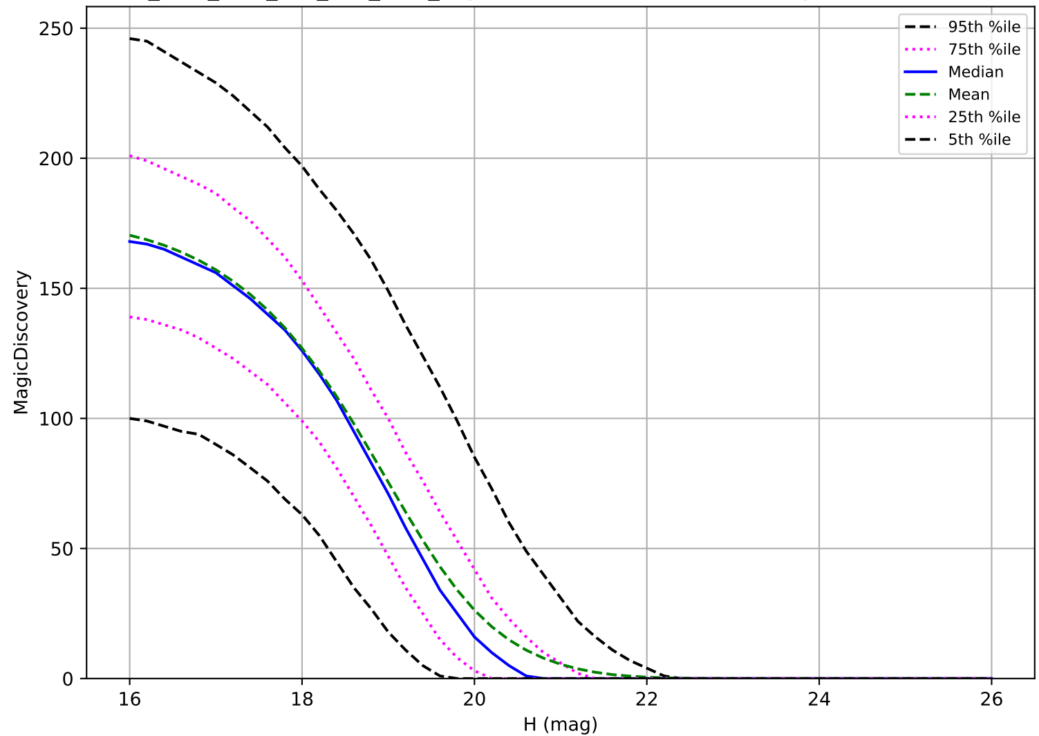
ddf_acor_sf20_lsf0_lsr0_v3.4_10yrs: MBA 6 detections in 60 nights detection loss
