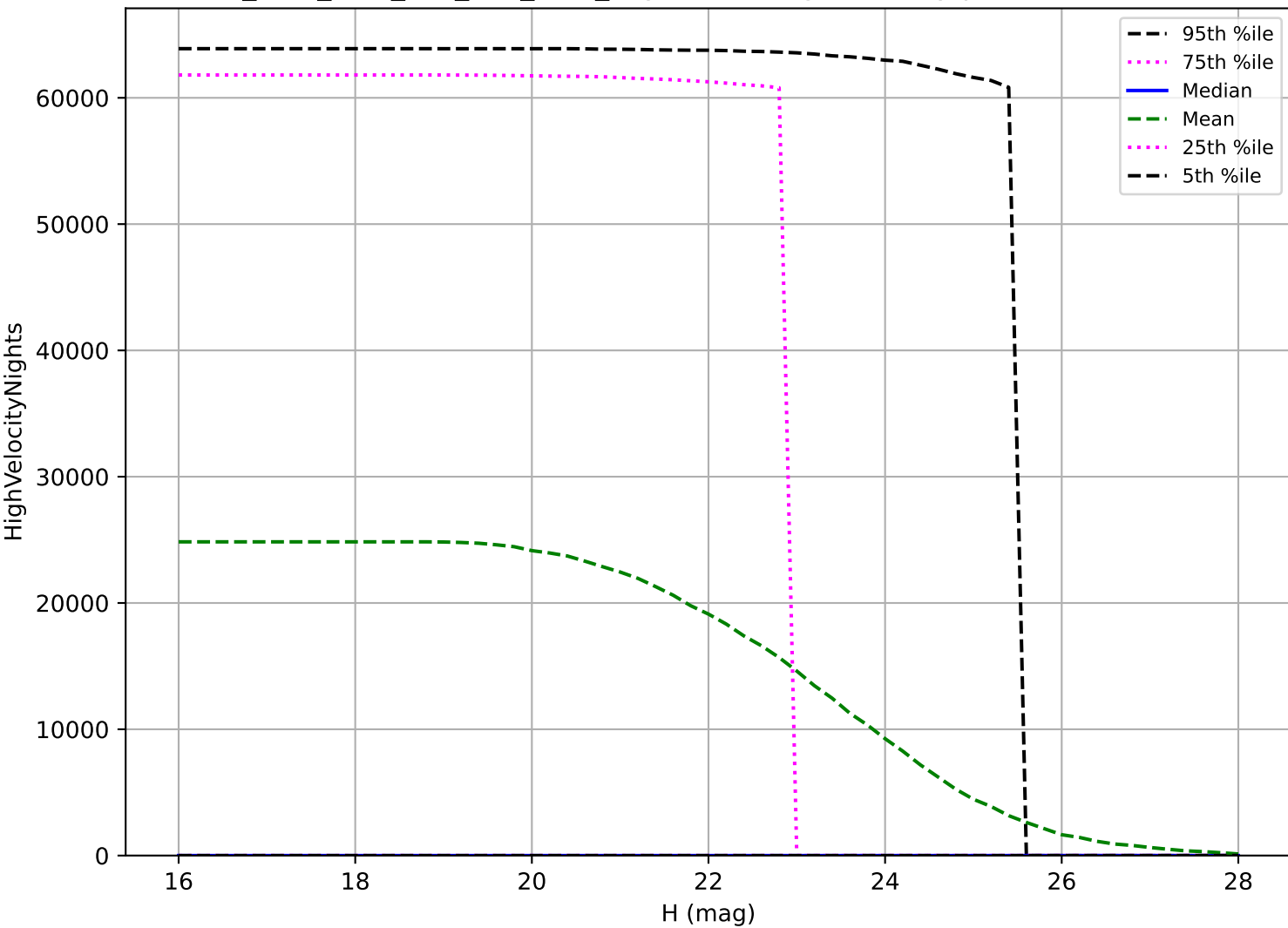
ddf_acor_sf20_lsf0_lsr0_v3.4_10yrs: PHA High velocity pair detection loss
