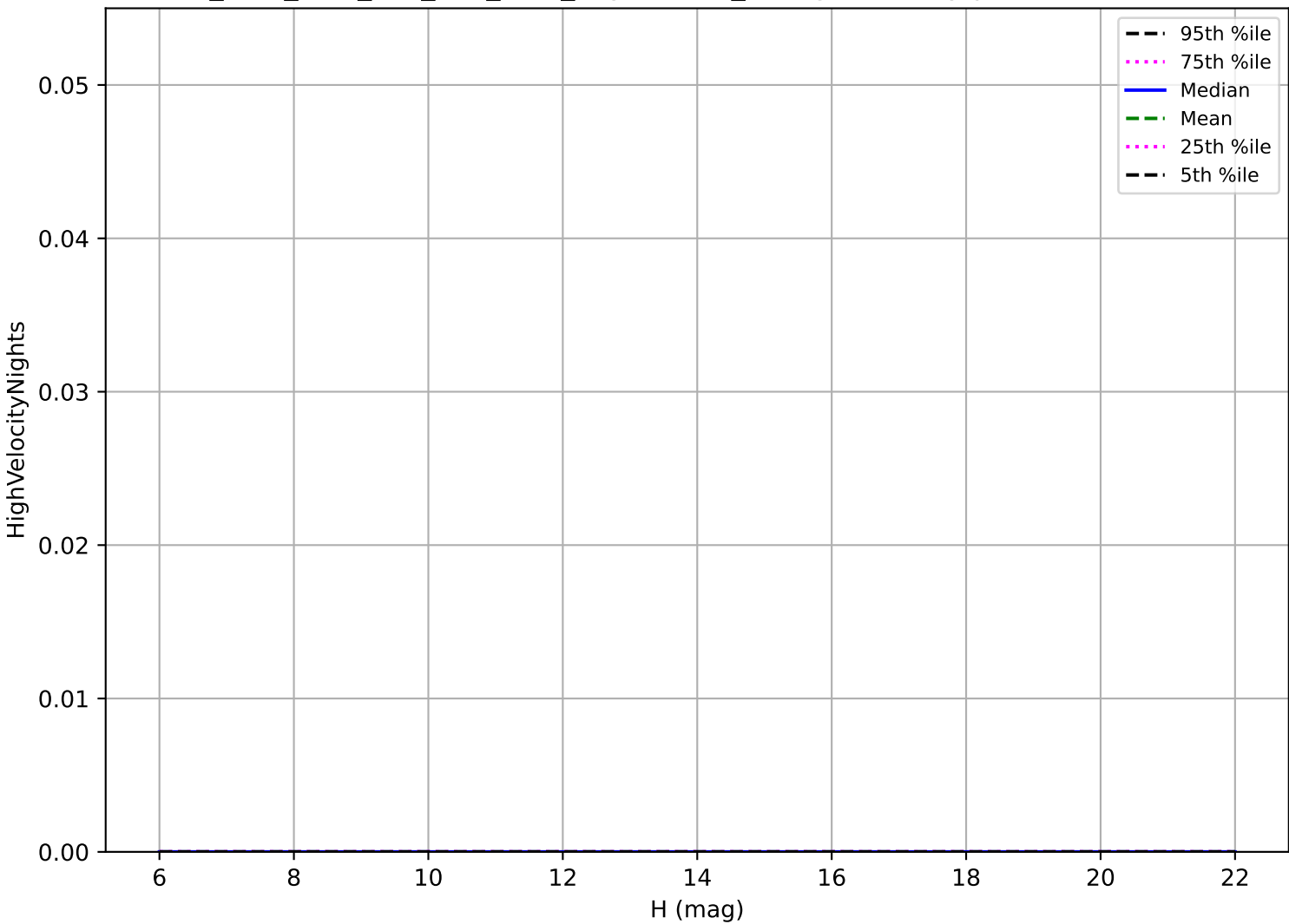
ddf_acor_sf20_lsf0_lsr0_v3.4_10yrs: OCC_r5 High velocity pair detection loss
