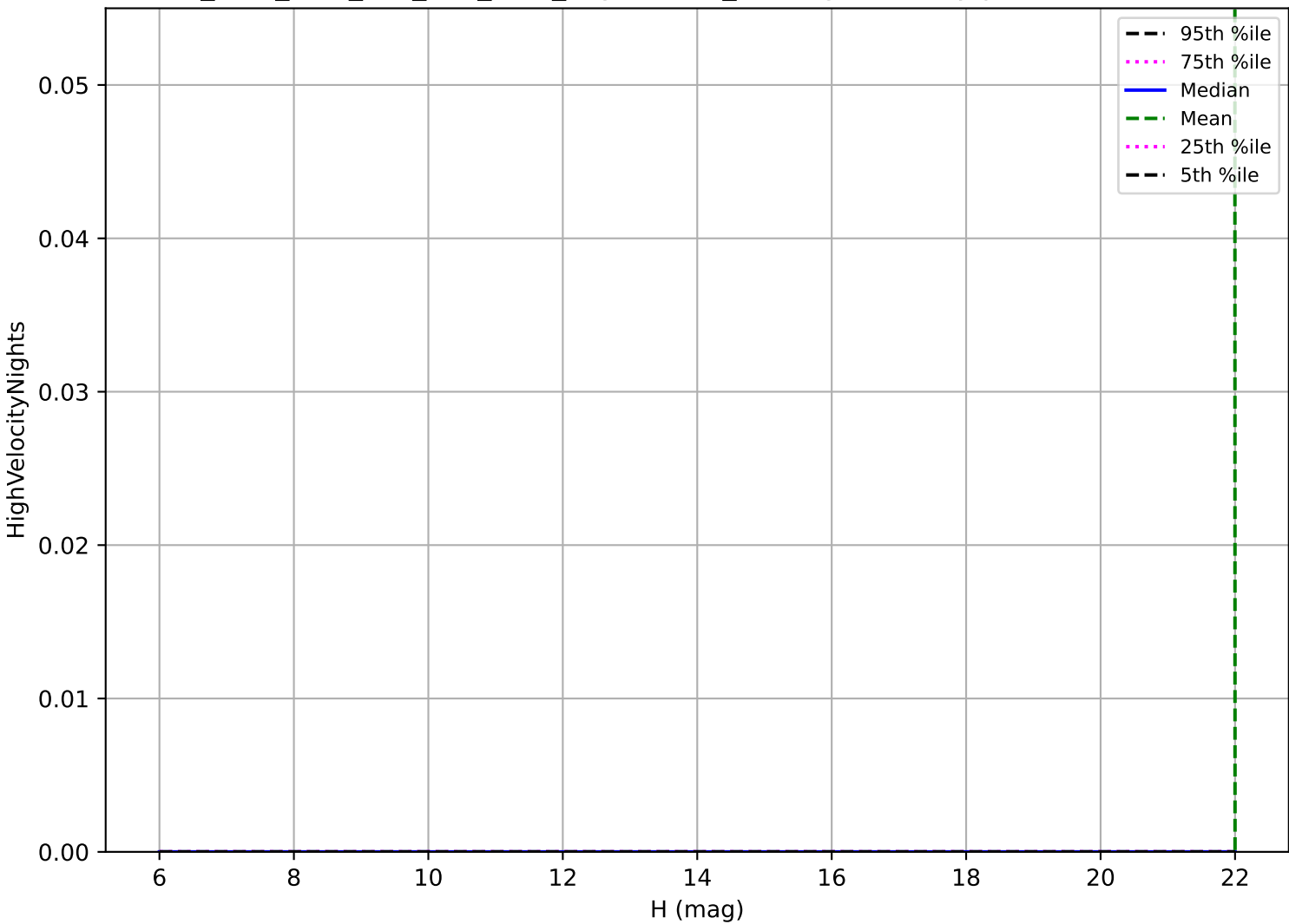
ddf_acor_sf20_lsf0_lsr0_v3.4_10yrs: OCC_r20 High velocity pair detection loss
