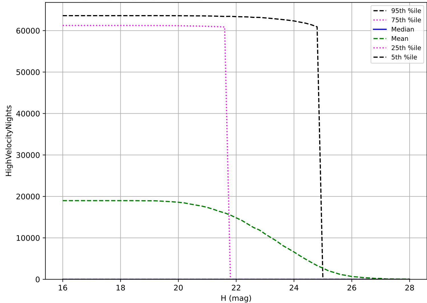
ddf_acor_sf20_lsf0_lsr0_v3.4_10yrs: NEO High velocity pair detection loss
