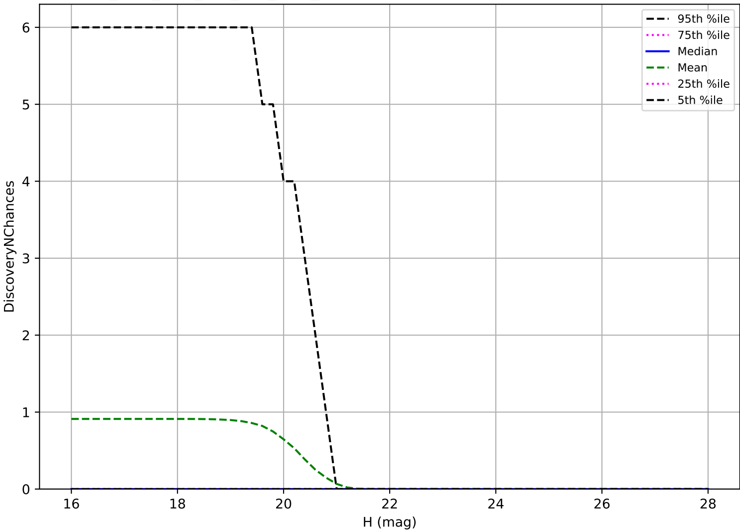
ddf_acor_sf20_lsf0_lsr0_v3.4_10yrs: Vatira 3 pairs in 15 nights detection loss
