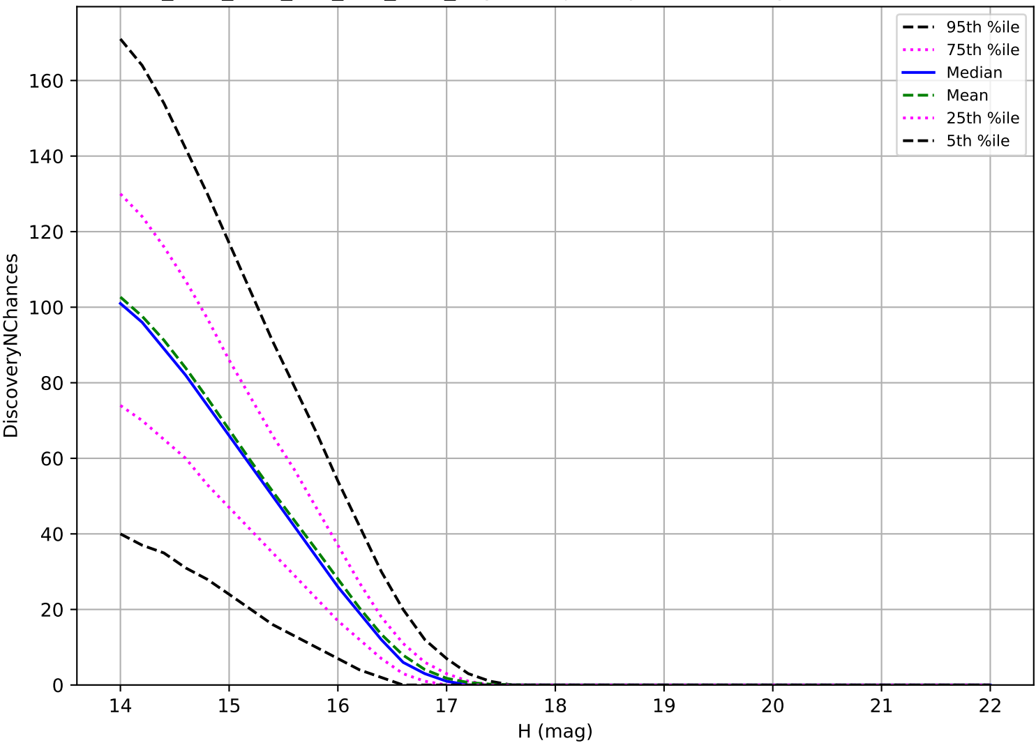
ddf_acor_sf20_lsf0_lsr0_v3.4_10yrs: Trojan 3 pairs in 15 nights detection loss
