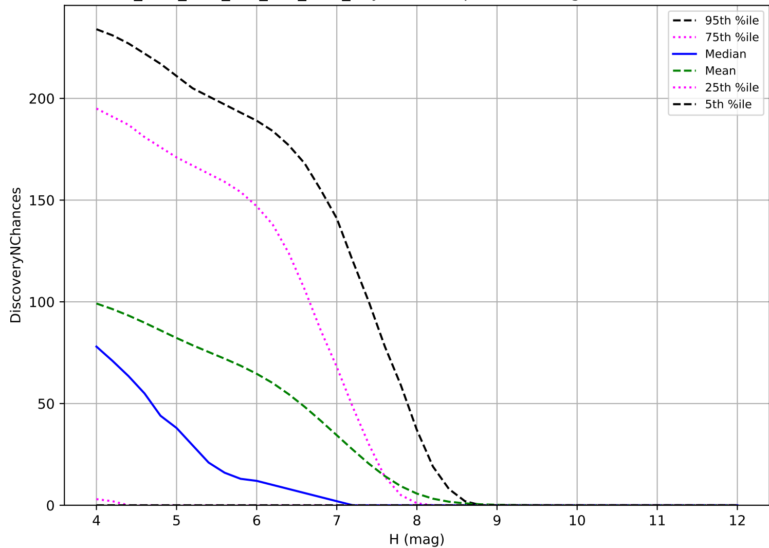
ddf_acor_sf20_lsf0_lsr0_v3.4_10yrs: TNO 3 pairs in 15 nights detection loss
