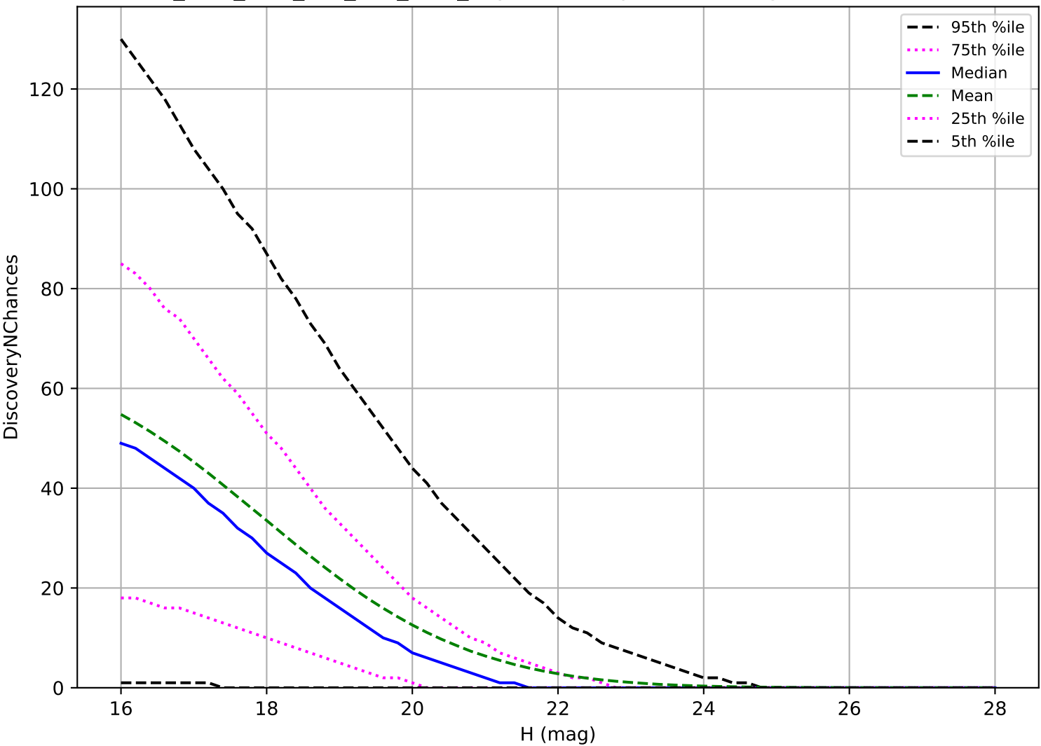
ddf_acor_sf20_lsf0_lsr0_v3.4_10yrs: PHA 3 pairs in 15 nights detection loss
