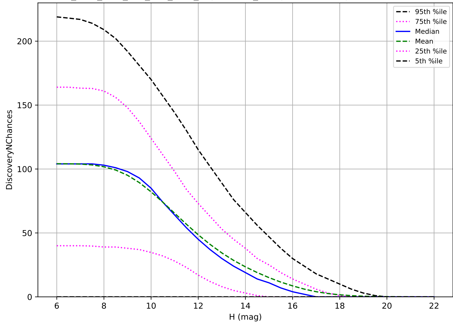
ddf_acor_sf20_lsf0_lsr0_v3.4_10yrs: OCC_r5 3 pairs in 15 nights detection loss
