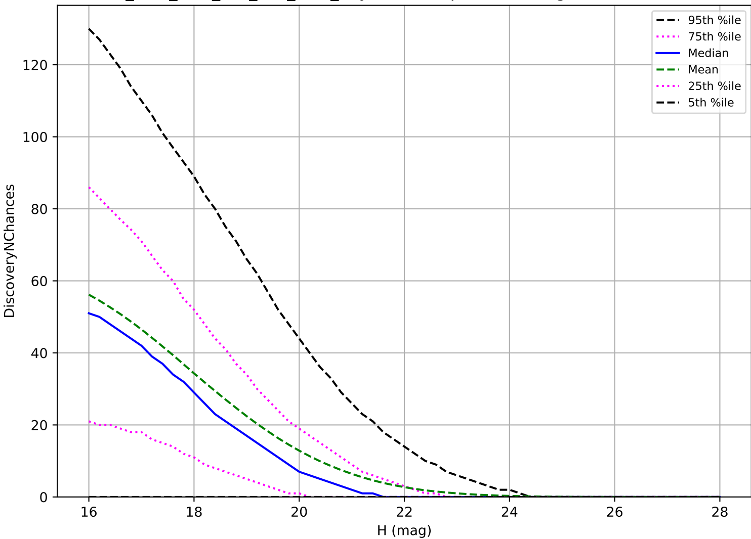
ddf_acor_sf20_lsf0_lsr0_v3.4_10yrs: NEO 3 pairs in 15 nights detection loss
