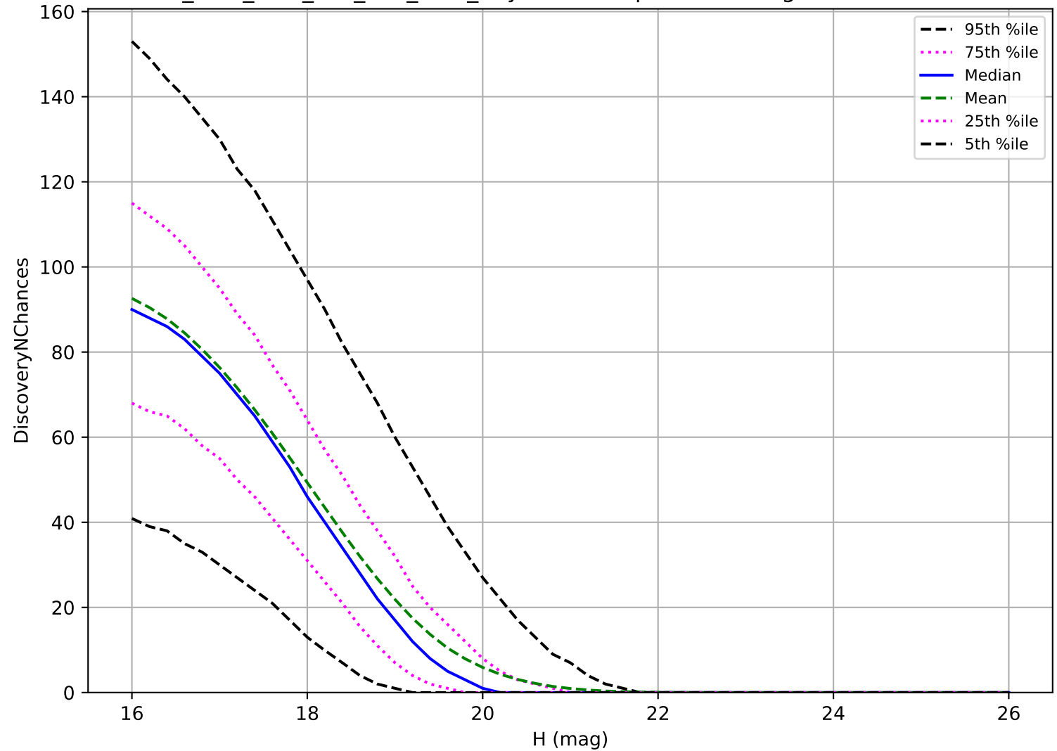
ddf_acor_sf20_lsf0_lsr0_v3.4_10yrs: MBA 3 pairs in 15 nights detection loss
