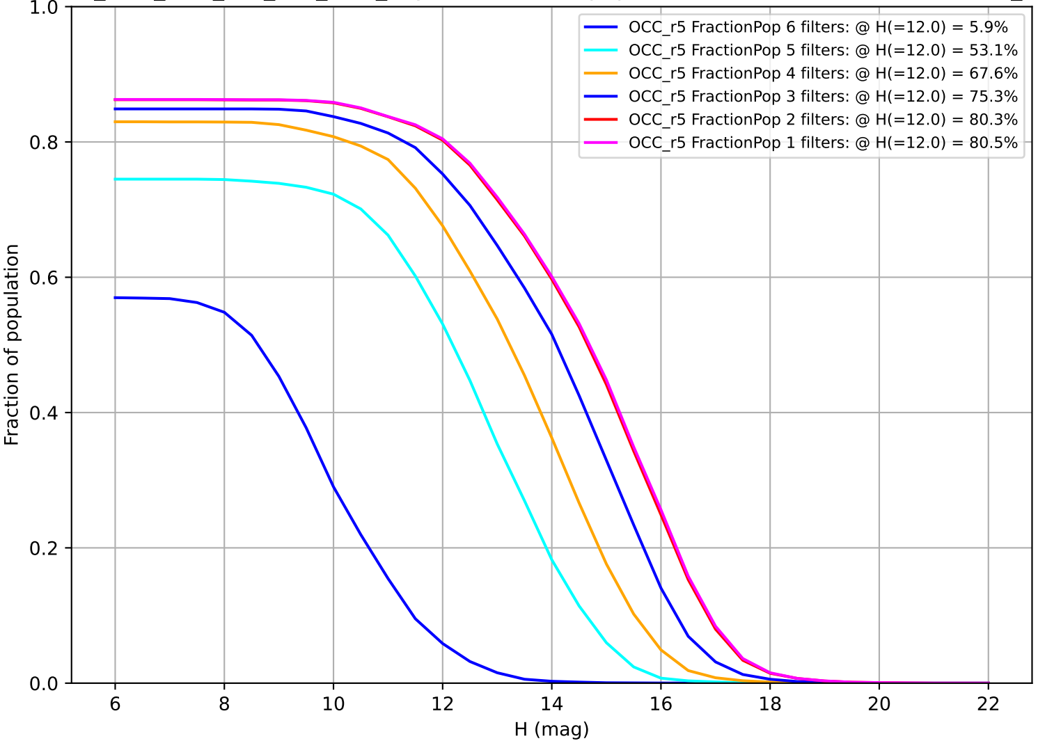
ddf_acor_sf20_lsf0_lsr0_v3.4_10yrs: Fraction of population with colors in X filters OCC_r5
