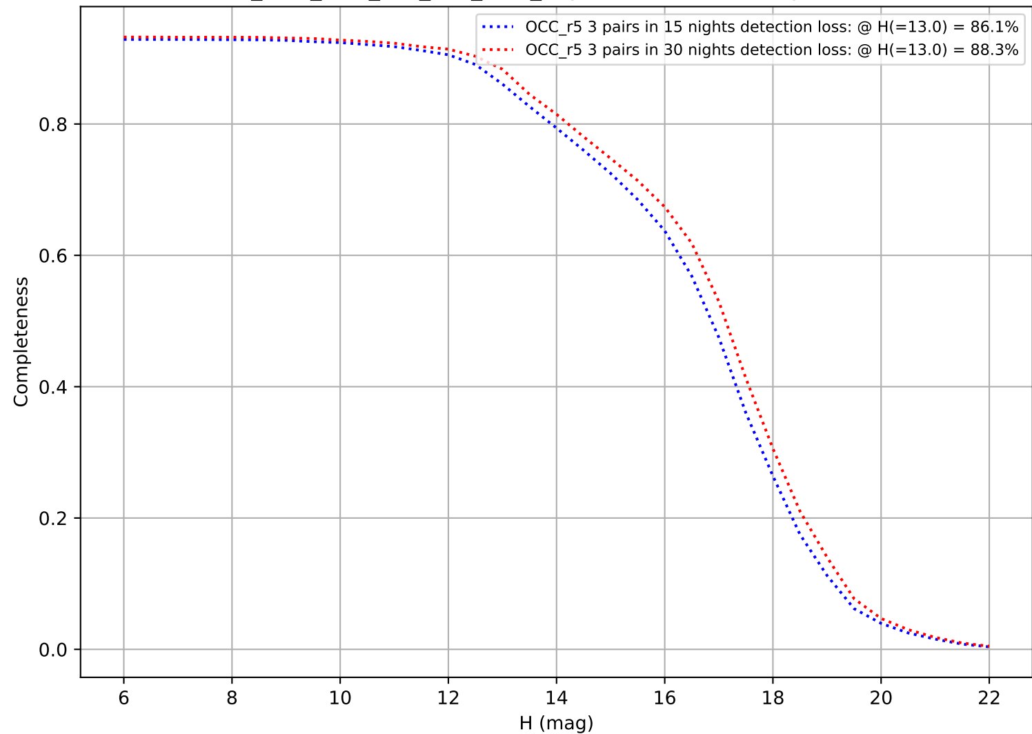
ddf_acor_sf20_lsf0_lsr0_v3.4_10yrs: DifferentialCompleteness
