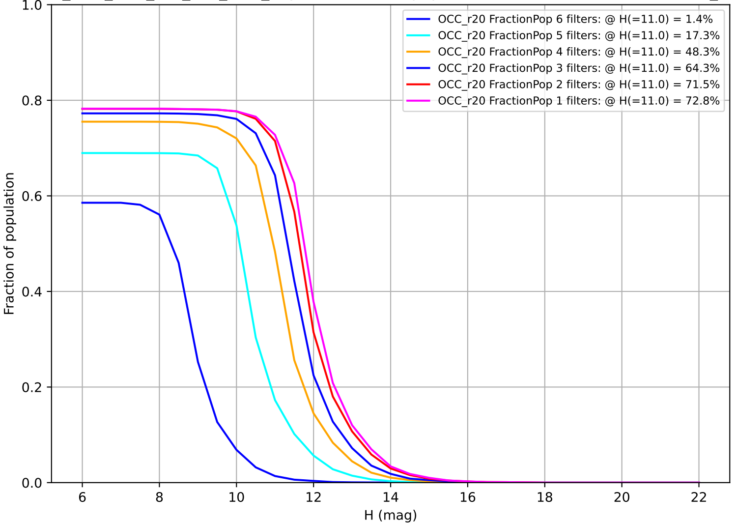
ddf_acor_sf20_lsf0_lsr0_v3.4_10yrs: Fraction of population with colors in X filters OCC_r20
