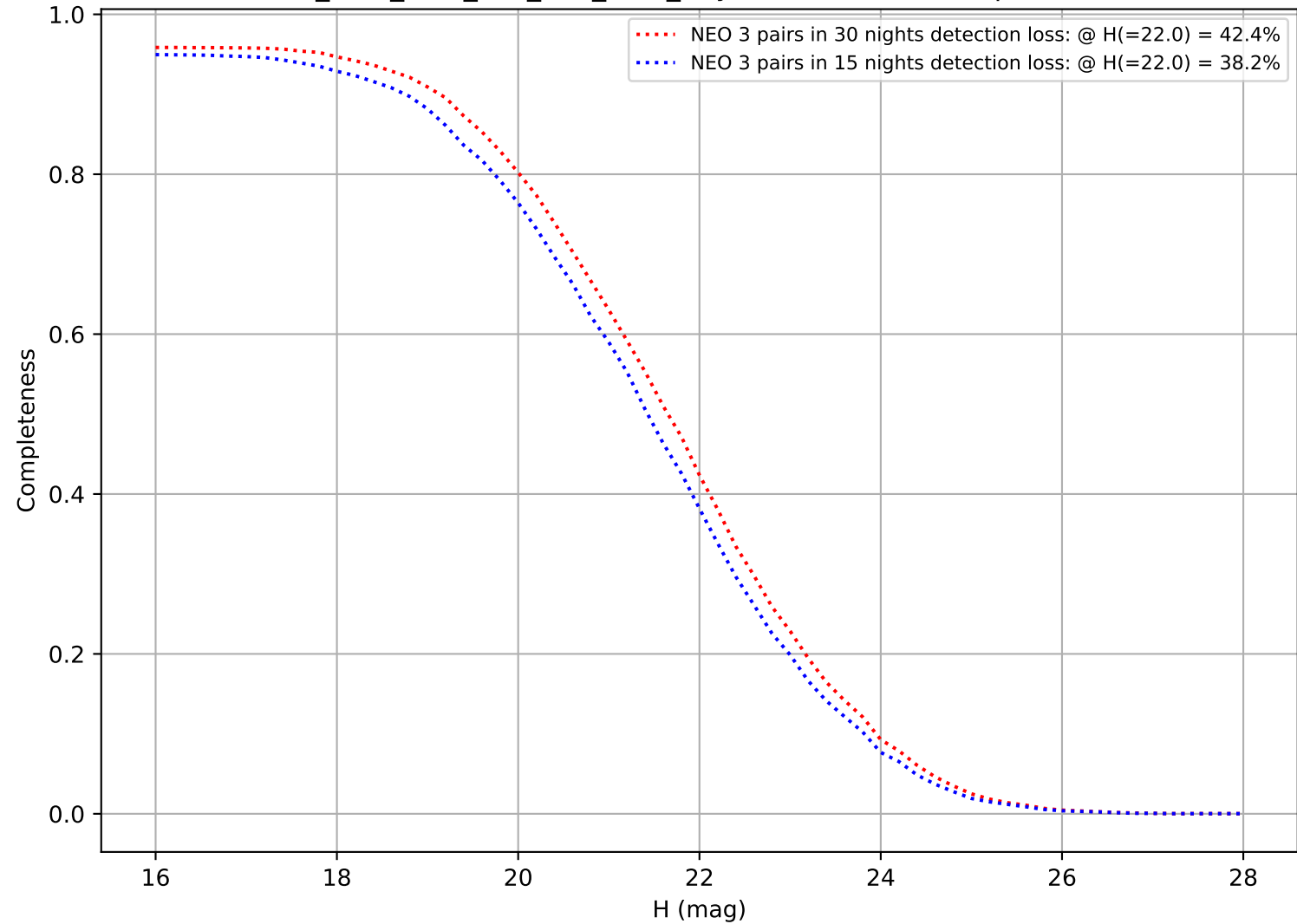
ddf_acor_sf20_lsf0_lsr0_v3.4_10yrs: DifferentialCompleteness
