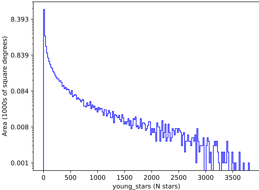
ddf_acor_sf20_lsf0_lsr0_v3.4_10yrs : young_stars
