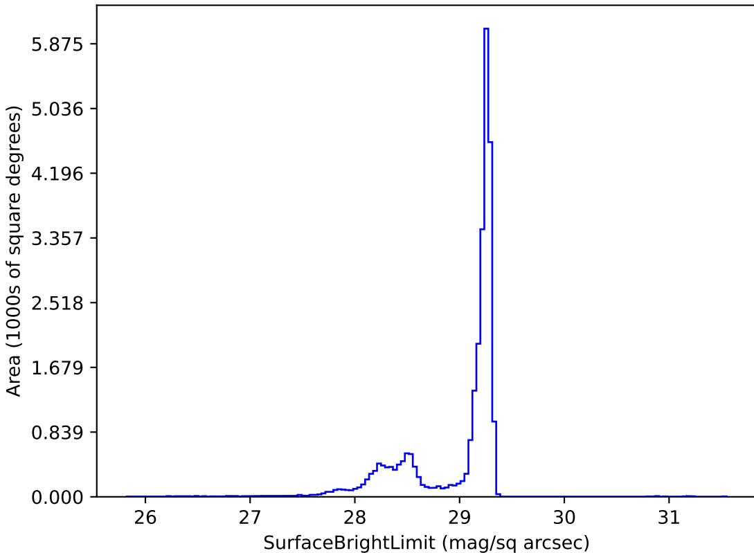
ddf_acor_sf20_lsf0_lsr0_v3.4_10yrs z: SurfaceBrightLimit
