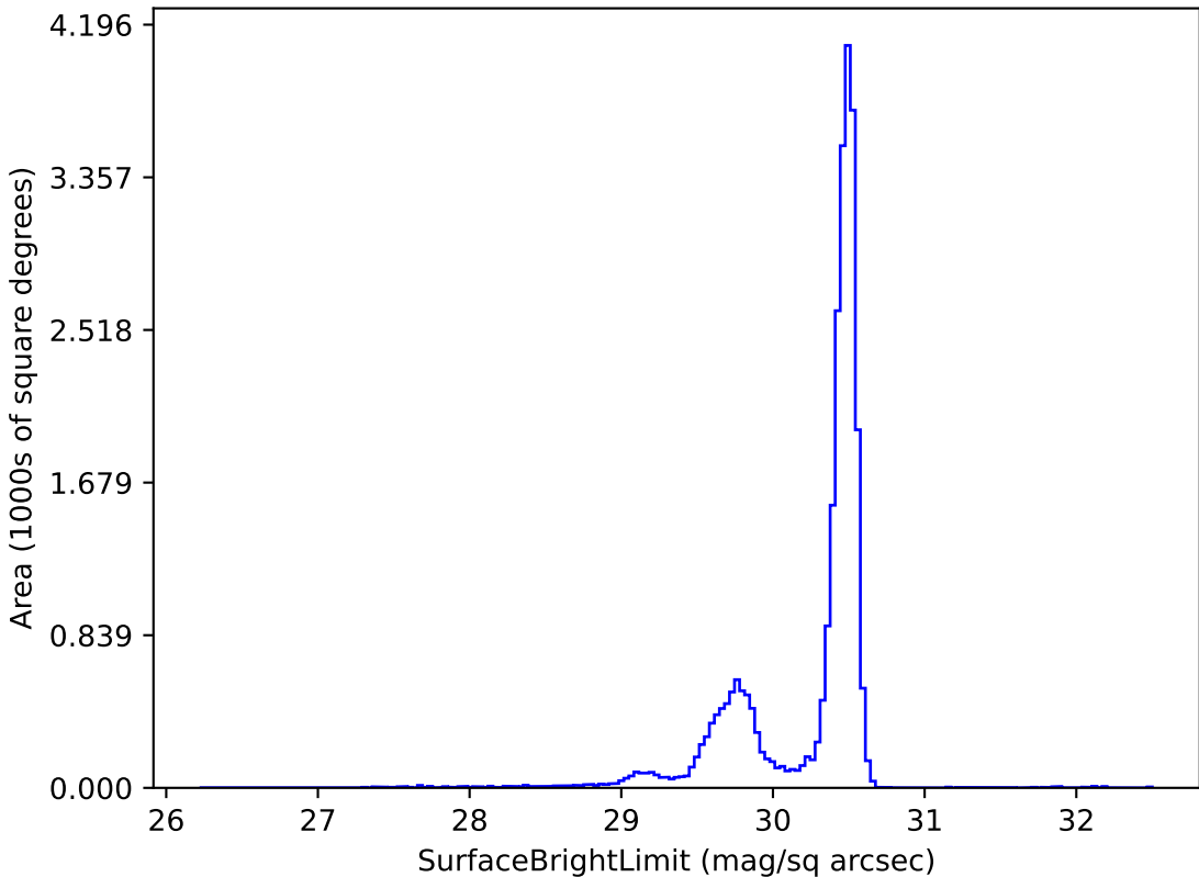
ddf_acor_sf20_lsf0_lsr0_v3.4_10yrs r: SurfaceBrightLimit
