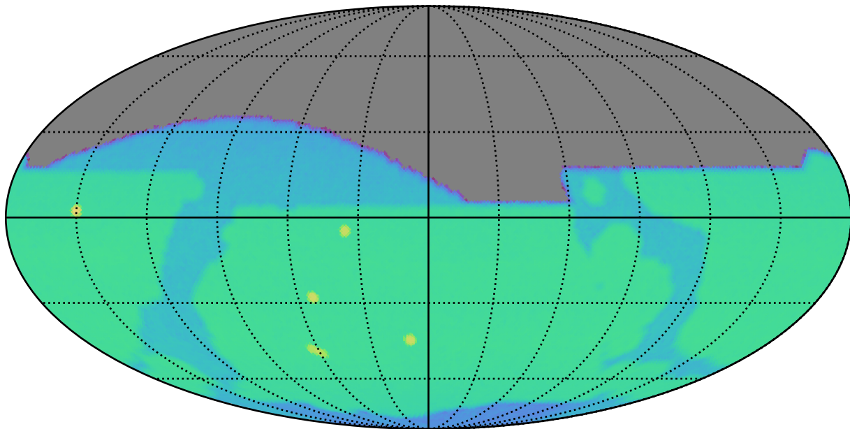
ddf_acor_sf20_lsf0_lsr0_v3.4_10yrs i: SurfaceBrightLimit
