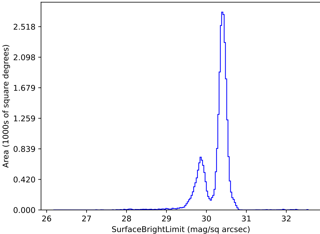
ddf_acor_sf20_lsf0_lsr0_v3.4_10yrs g: SurfaceBrightLimit
