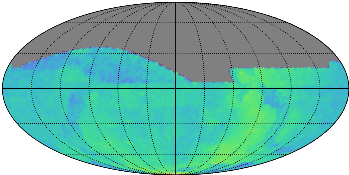
ddf_acor_sf20_lsf0_lsr0_v3.4_10yrs : Parallax Coverage @ 24.0
