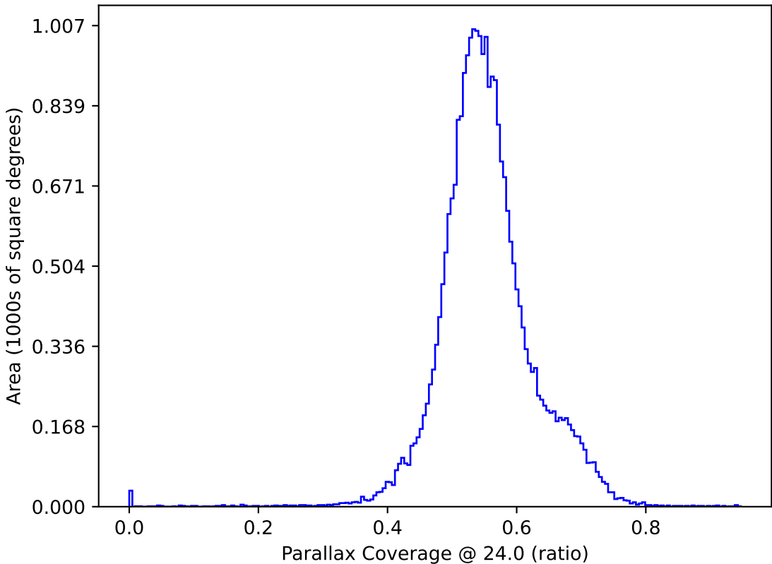
ddf_acor_sf20_lsf0_lsr0_v3.4_10yrs : Parallax Coverage @ 24.0
