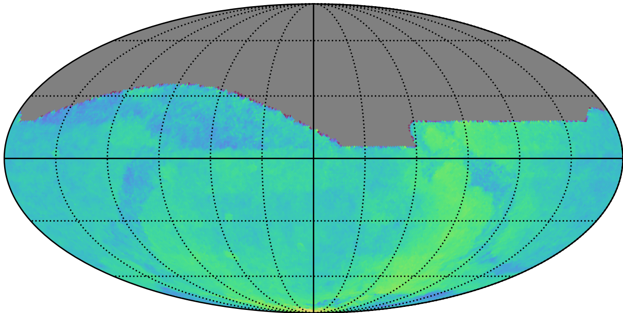
ddf_acor_sf20_lsf0_lsr0_v3.4_10yrs : Parallax Coverage @ 22.4
