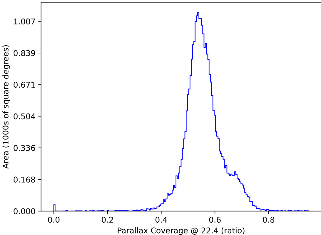
ddf_acor_sf20_lsf0_lsr0_v3.4_10yrs : Parallax Coverage @ 22.4
