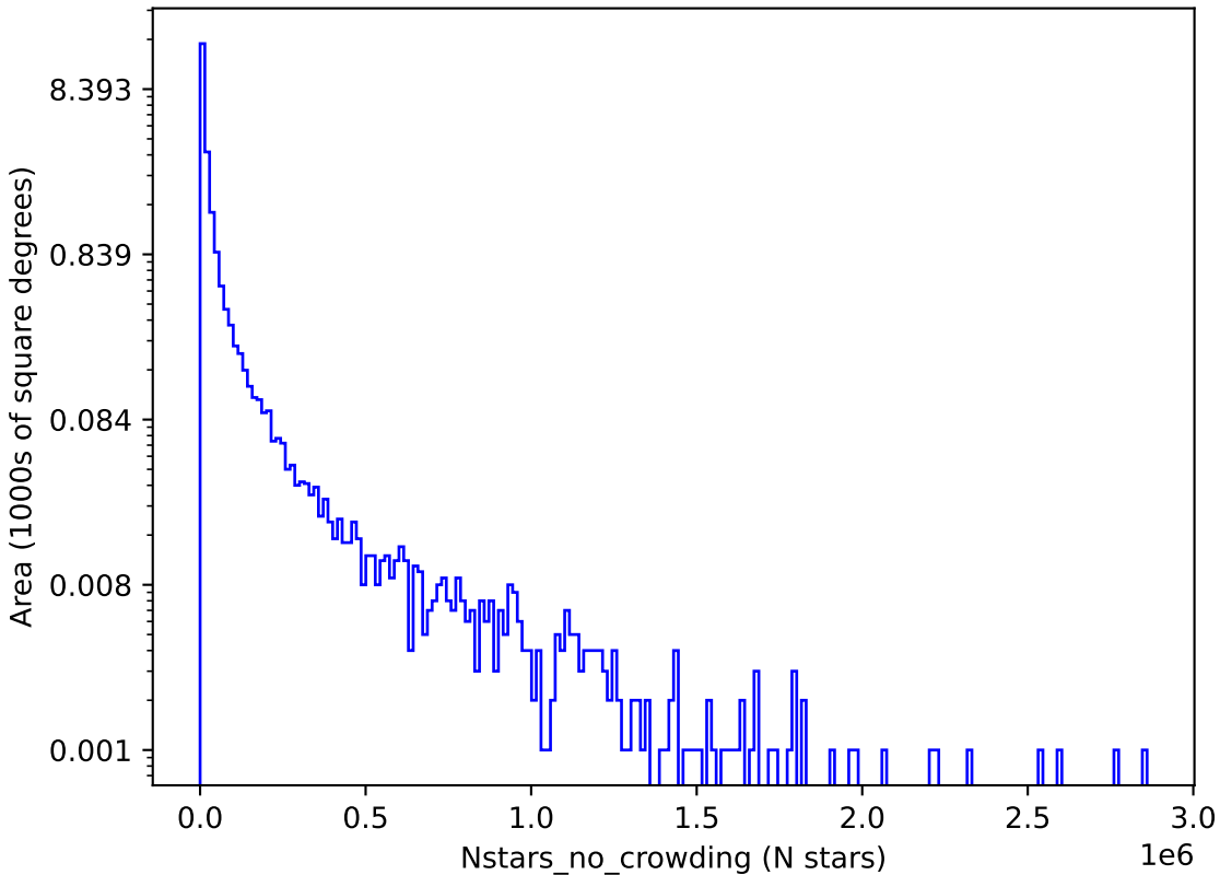
ddf_acor_sf20_lsf0_lsr0_v3.4_10yrs u: Nstars_no_crowding
