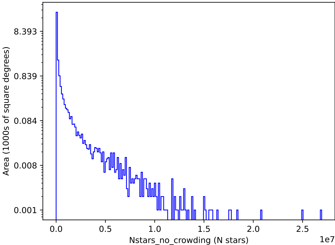
ddf_acor_sf20_lsf0_lsr0_v3.4_10yrs i: Nstars_no_crowding
