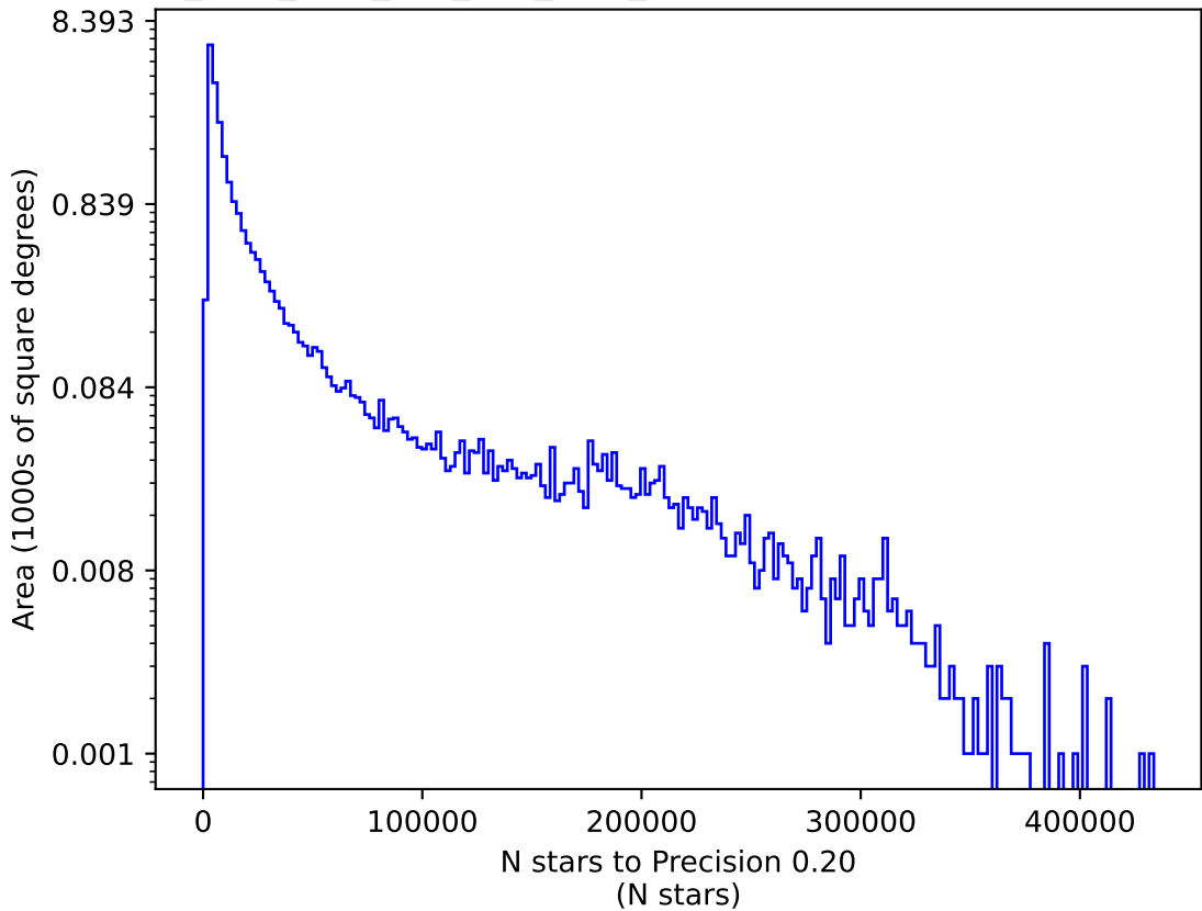
ddf_acor_sf20_lsf0_lsr0_v3.4_10yrs u: N stars to Precision 0.20
